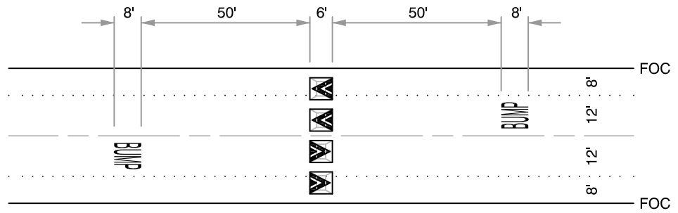
ASPHALT CONCRETE SPEED CUSHION
