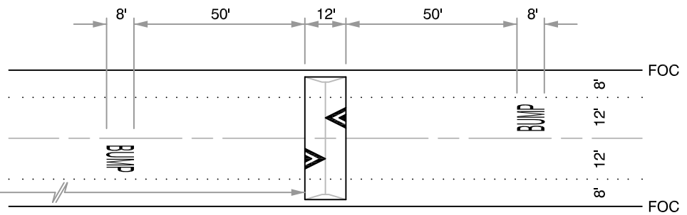
ASPHALT CONCRETE SPEED HUMP
